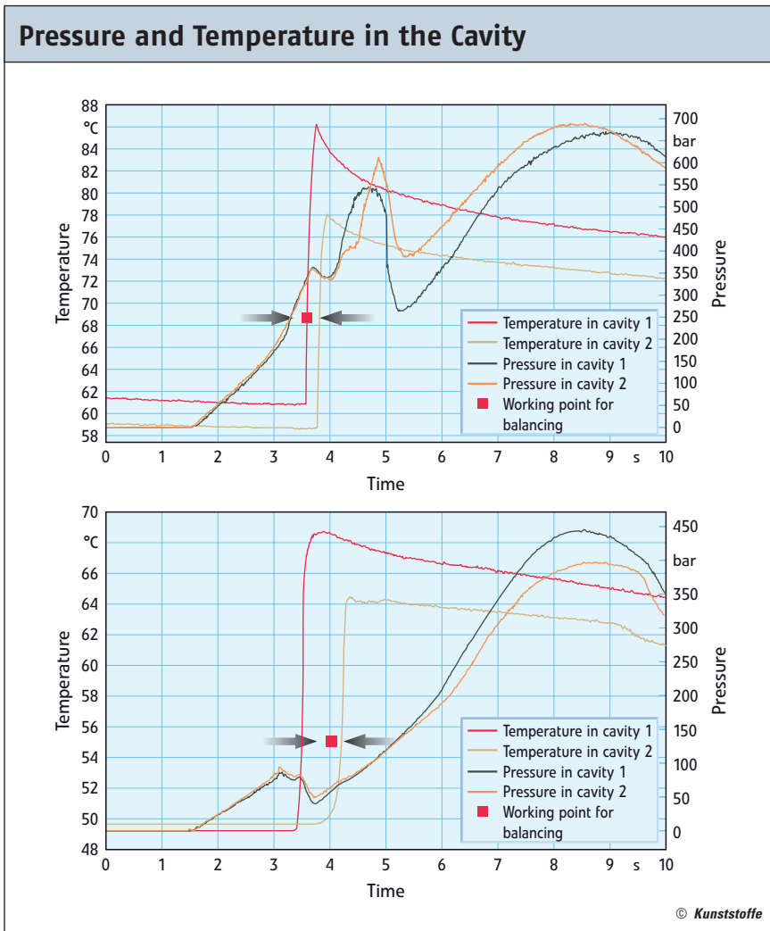
Fig. 1. Cavity pressure curves and cavity temperatures for a 2-cavity mold at different machine settings. The shape of the mold-wall temperature is always unambiguous and can therefore be detected automatically and used for controlling or balancing the hot runners (figure: Priamus)
