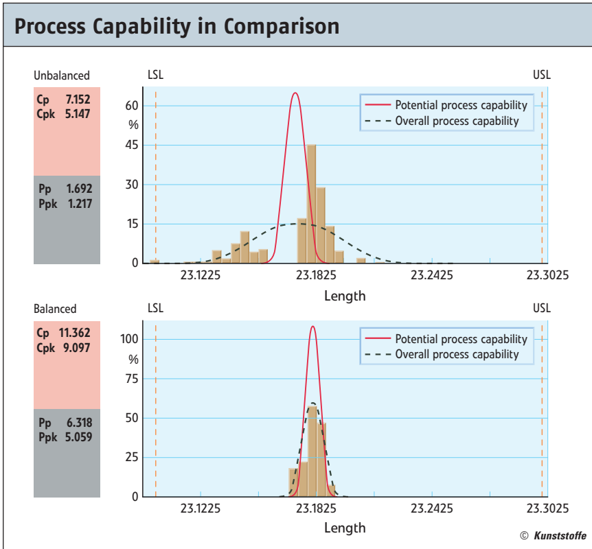
Fig. 4. Potential process capability and overall process capability, expressed in terms of the length of the sintered ceramic bodies. This overall process capability improves from the unbalanced to the balanced state by more than a factor of 4 (figure: Philips)
