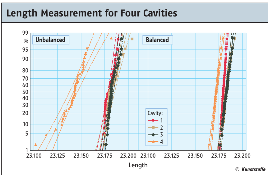
Fig. 5. Probability paper for the total length of the sintered parts in the balanced and unbalanced process. In the ideal case of a normal distribution, the values lie on a straight line. In the unbalanced state, one of the cavities does not follow this distribution, because it was not fully injected. A similar picture is presented by an analysis of the weight (not shown) (figure: Philips)
