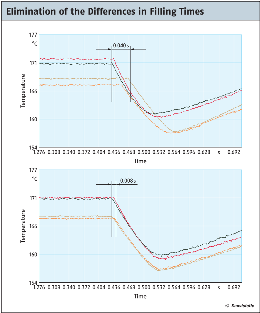
Fig. 7. Cavity temperature signals for a 4-cavity LSR injection mold in the balanced and unbalanced states. The Priamus Fill System compensated the different filling times with the aid of automatically calculated delay times at the needle valves (figure: Priamus)
