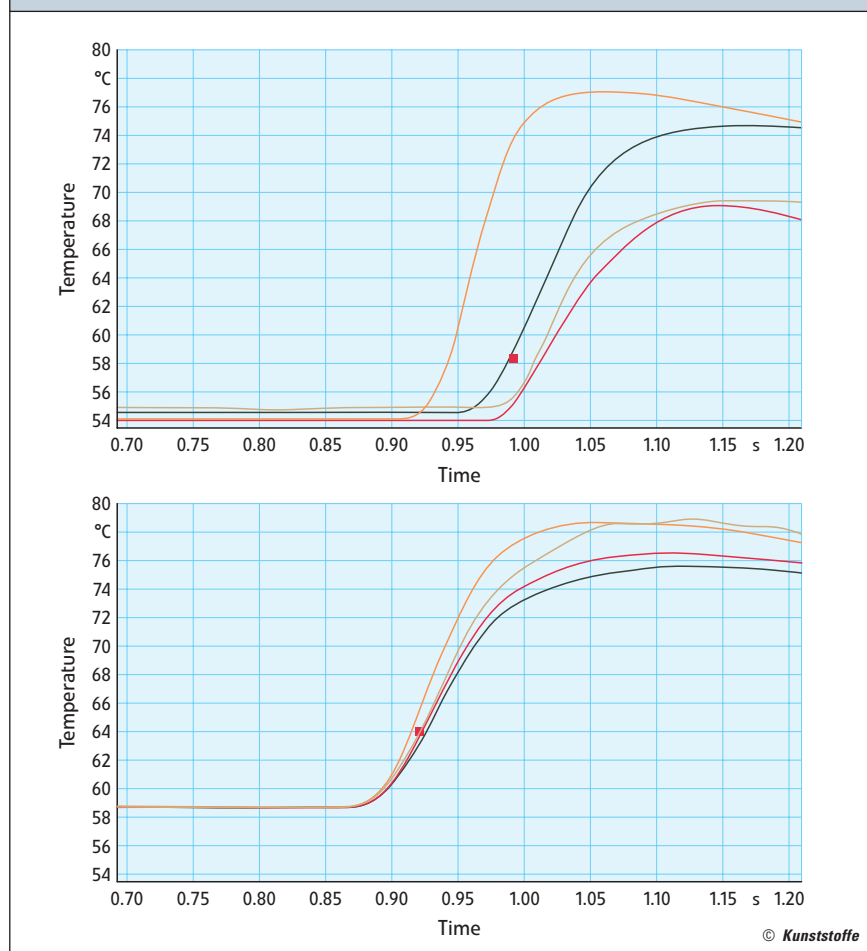
Fig. 3. Differences in filling times of the various cavities before and after balancing, as shown by curves of the cavity temperature. The nozzle temperatures of the hot-runner system are automatically changed such that each cavity is filled at the same time (figure: Priamus)
